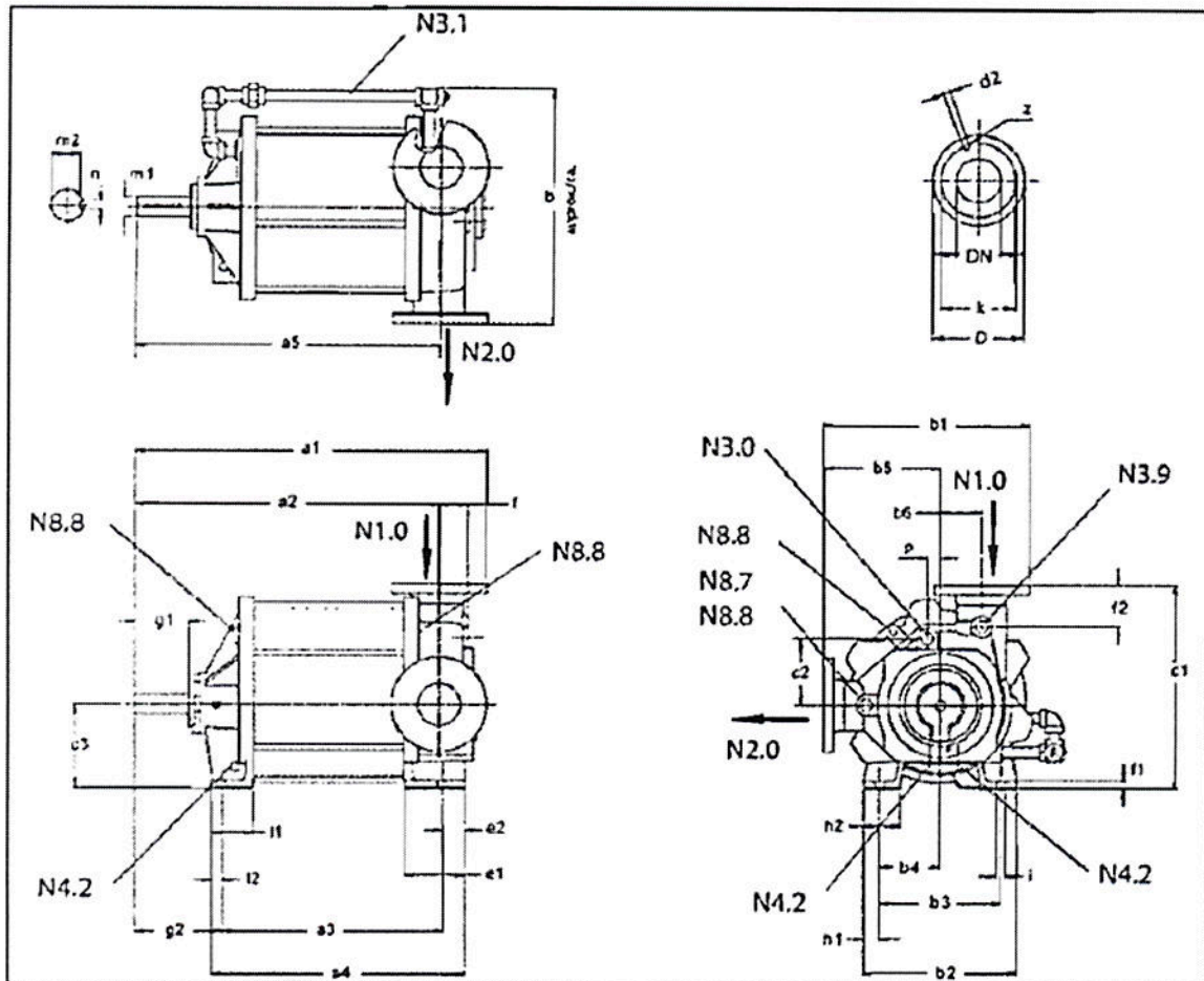
Fig. 1: Dimensions of Vectra GL
